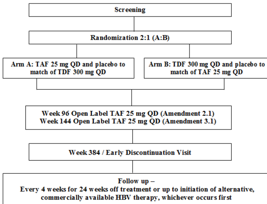
Figure 3-1. Study Schema
